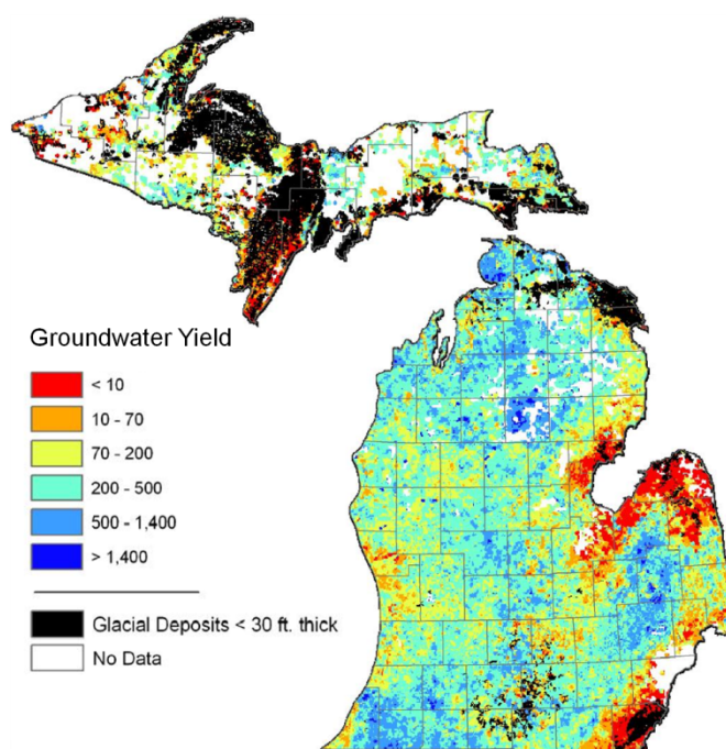
Figure 5. The estimated groundwater yield from glacial deposits in Michigan. The colors indicate how quickly groundwater could be pumped out. This rate is expressed in gallons per minute (gpm) 9
